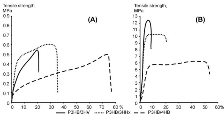
Figure 4. Tensile strength: A – randomly oriented ultrafine fibers, B – aligned oriented ultrafine fibers produced by electrospinning from solutions of PHAs with different chemical compositions: a – P(3HB); b – P(3HB-co-10.5 mol.%-3HV); c – P(3HB-co-10.0 mol.%-4HB); d – (3HB-co-10.0 mol.%-3HHx).
